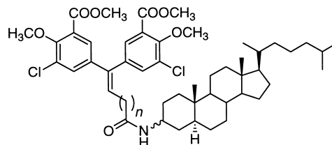
18 , n = 0, 3 \beta 19 , n = 0, 3 \alpha 20 , n = 1, 3 \beta 21 , n = 1, 3 \alpha
