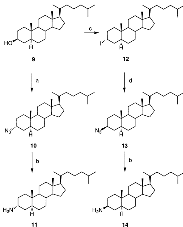
Scheme 1. Reagents and conditions: (a) PPh_3 , DEAD, (PhO)_2PON_3 , THF, 25 °C, 24 h, 51%; (b) LiAlH_4 , Et_2O , reflux, 11 : 65%; 14 : 69.7%; (c) PPh_3 , DEAD, CH_3I , THF, 25 °C, 76%; (d) NaN_3 , DMSO, 90 °C, 5 h, 81%.
