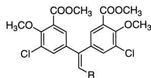
15 , R = COOH 16 , R = CH 2 CH 2 OH 17 , R = CH 2 COOH
